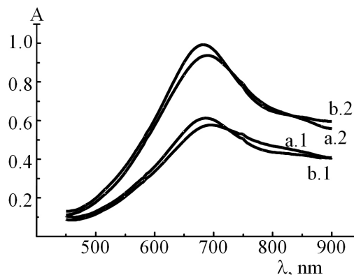
Fig. 2. Absorption spectra of HPB obtained by the reduction of 18-MPC with Asc in the presence of Bi(III).
